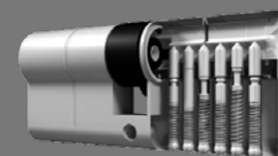
Locking Cylinder
